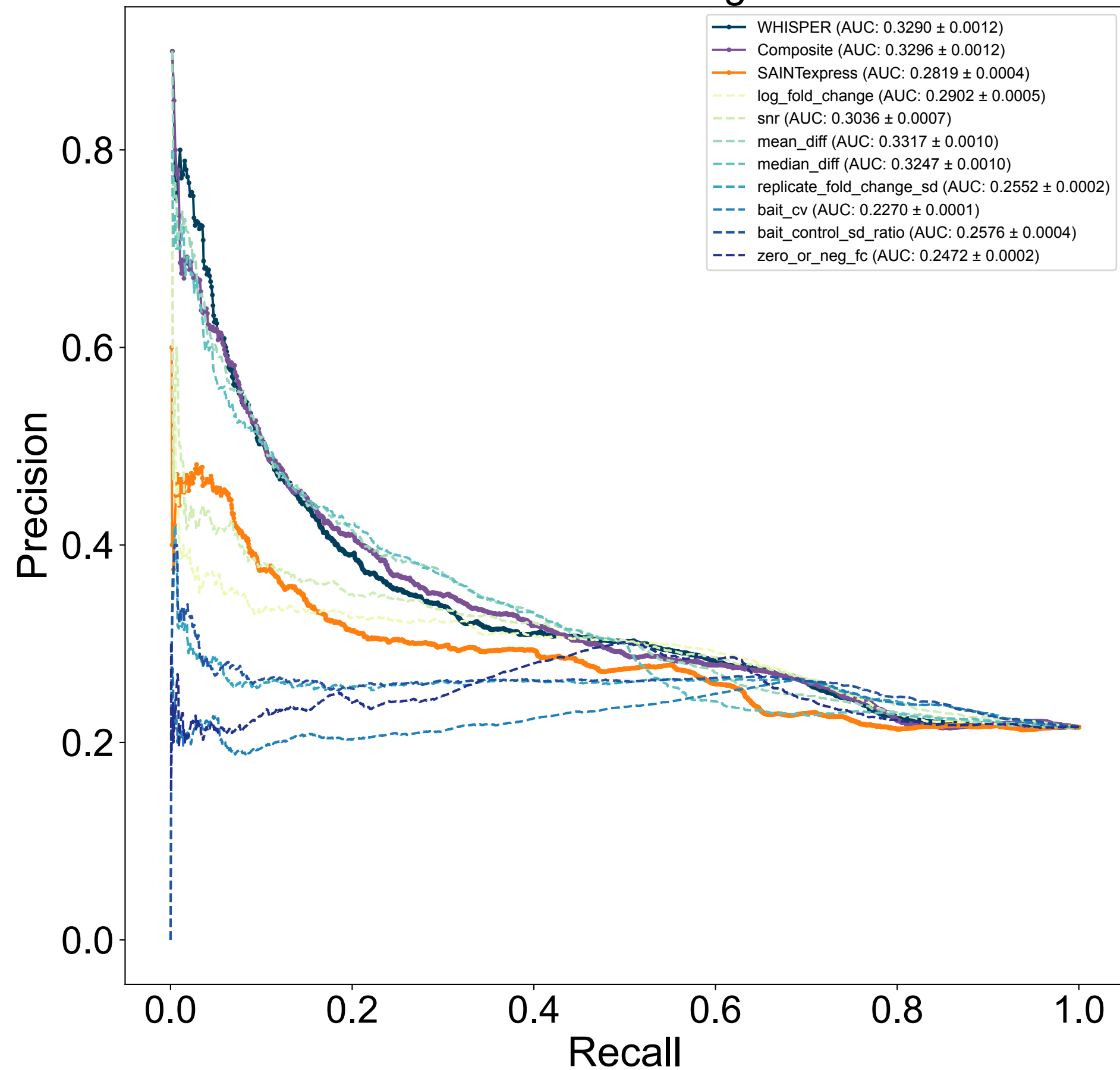
Precision–Recall Curve Including Individual Features
